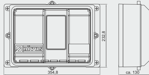
Field enclosure
