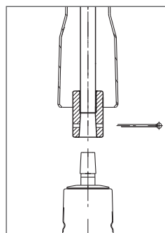
Slide back outer protecting tube, remove split pin
