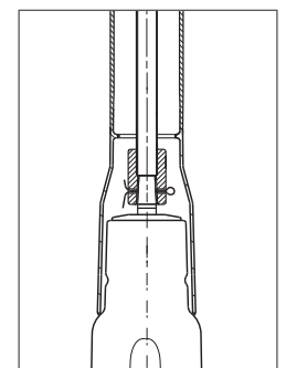
Slide outer protecting tube over gate valve housing
