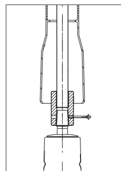
Place extension spindle shaft over valve spindle
