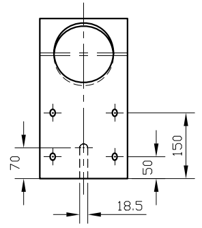
Slot for the M12 screws
